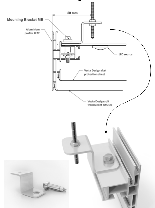
Suspension with Mounting Bracket MB
