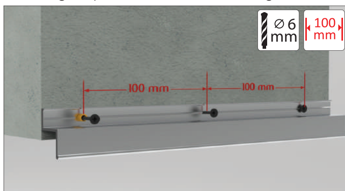
Fastening the profile to the concrete ceiling
