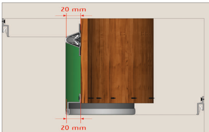
Fastening the profile to the concrete ceiling
