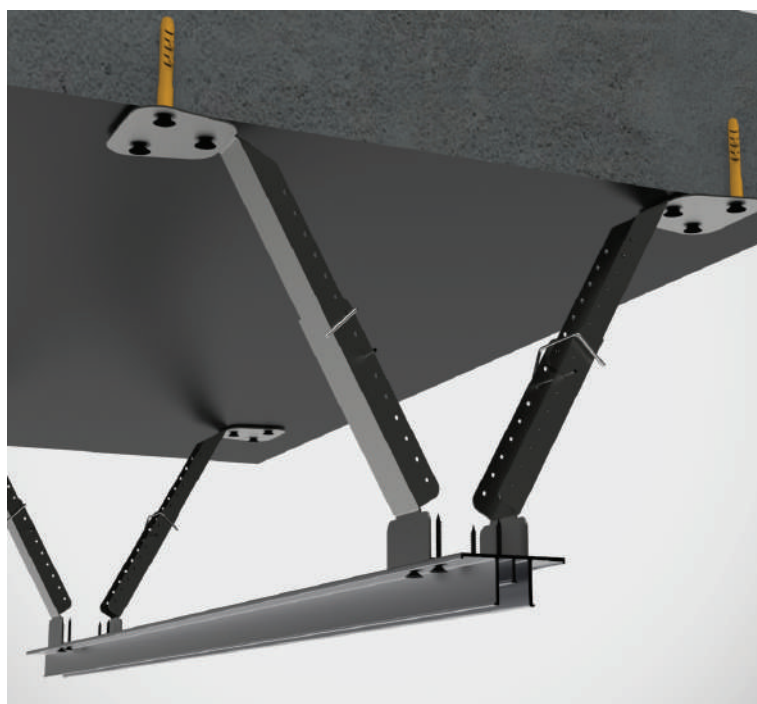
Installation of profile to the base ceiling using Vecta Design support ceiling system
