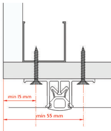
Cross-section of fastening the profile
