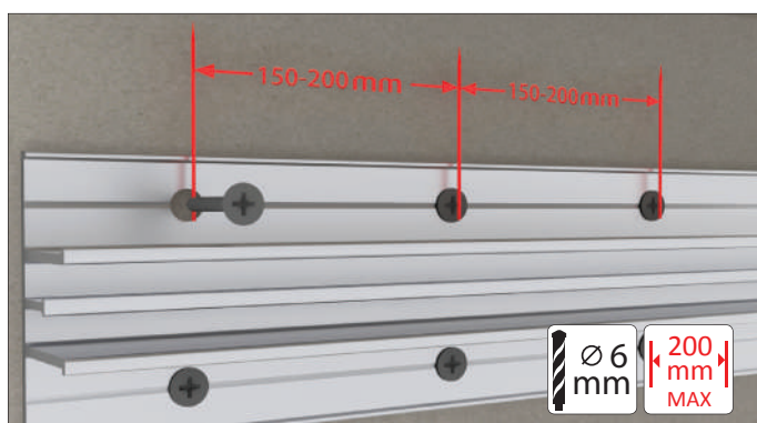
Fastening the profile to the plasterboard surface
