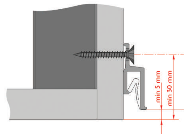
Cross-section of fastening the profile
