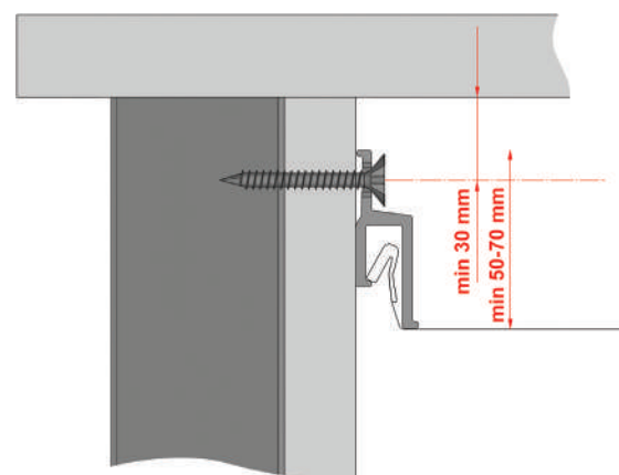
Cross-section of fastening the profile
