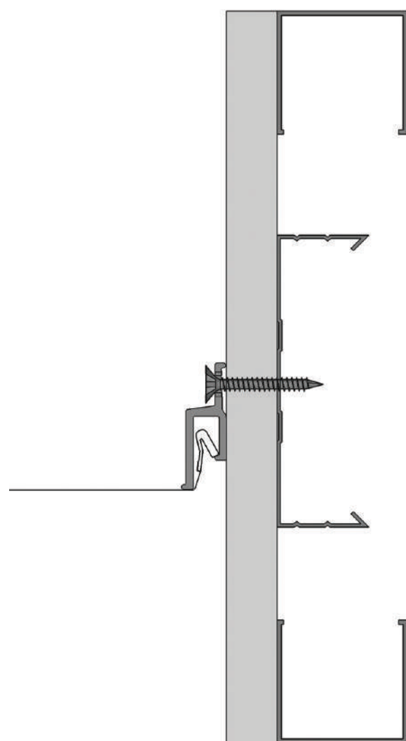
Cross-section of fastening the profile
