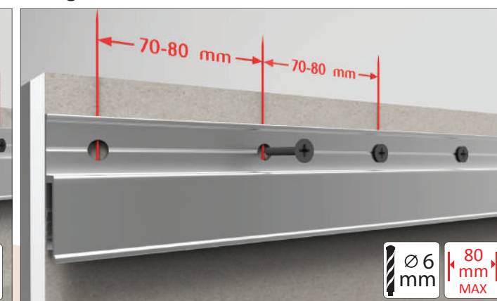
Fastening the profile to the plasterboard wall or ceiling
