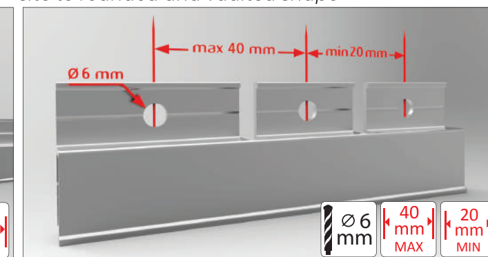
Pre-notched in the factory for easy adaptation on site to rounded and vaulted shape
